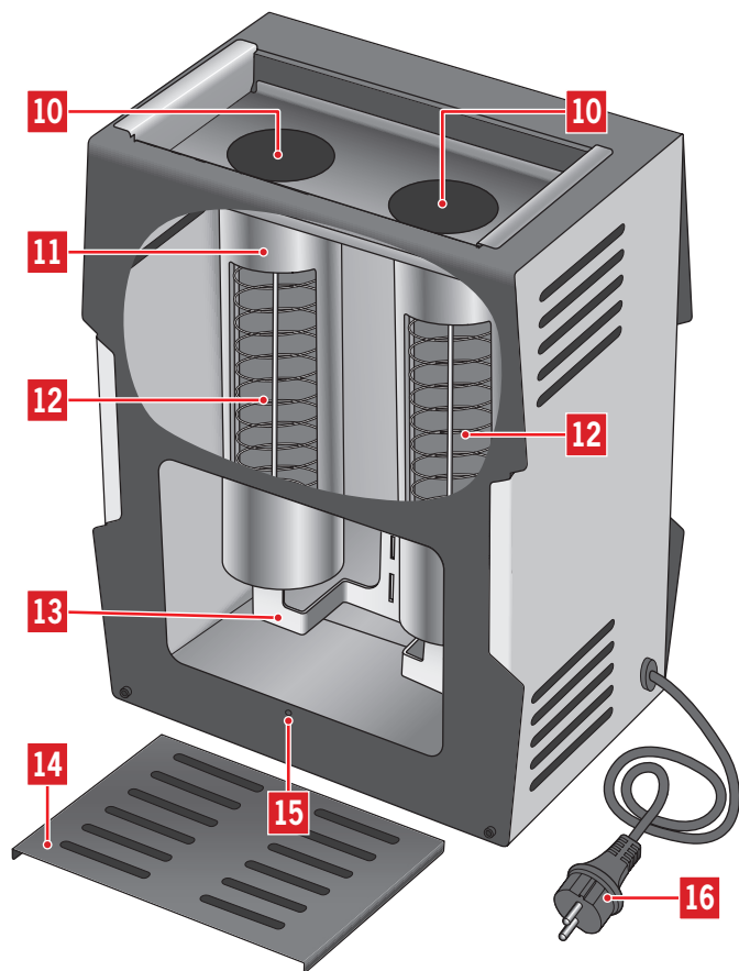
Fig. 2: Rear view and interior components (cross-sectional view)
