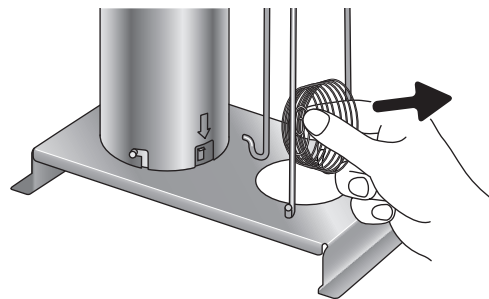
Fig. 6: Removing the springs
